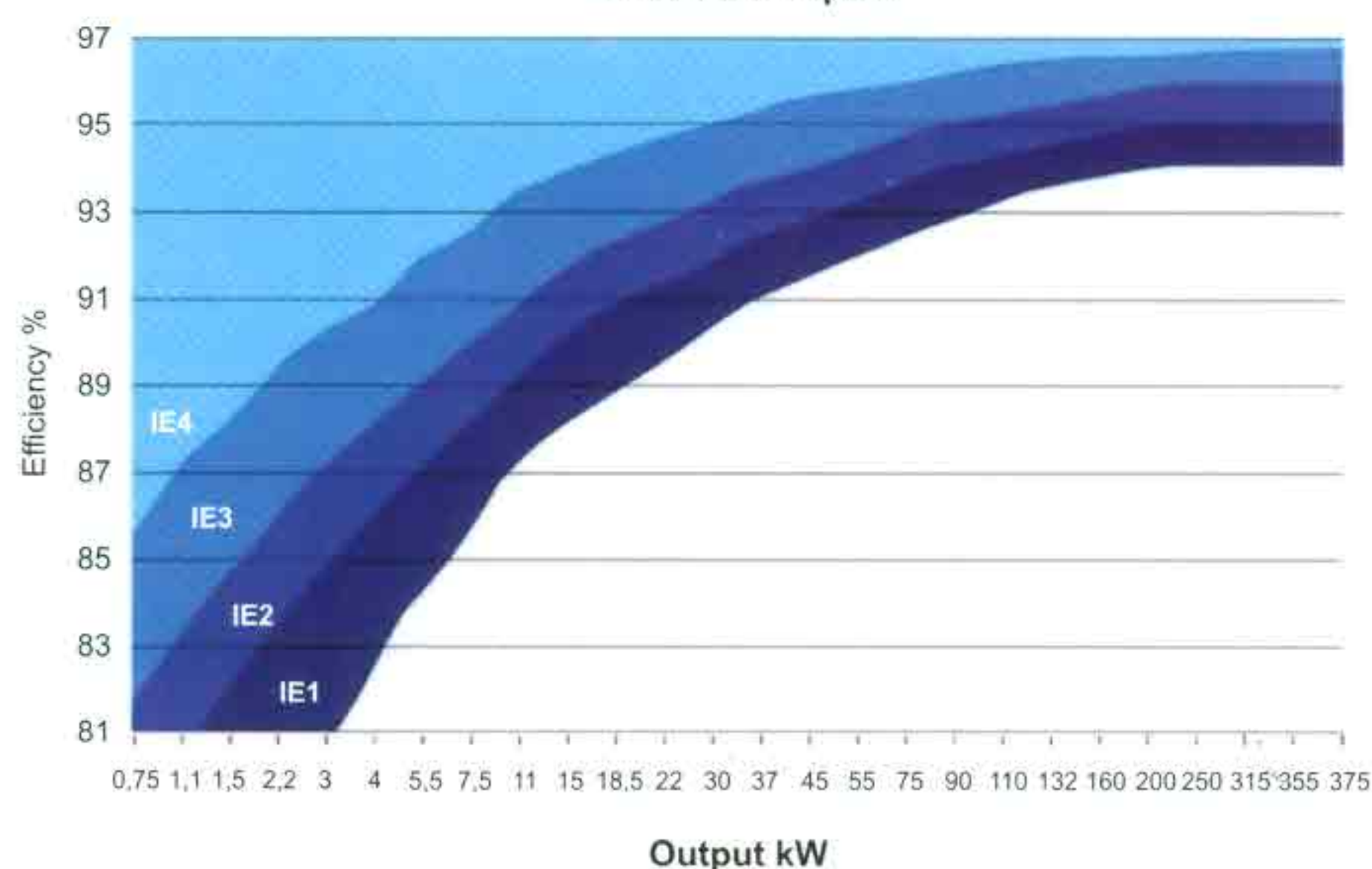
IE Classes - 4 pole
